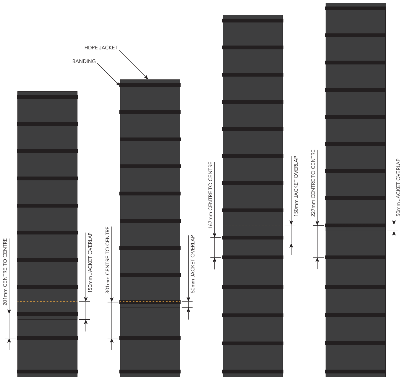
Fig. 7: Correct banding positions for multiple jacket assemblies.
